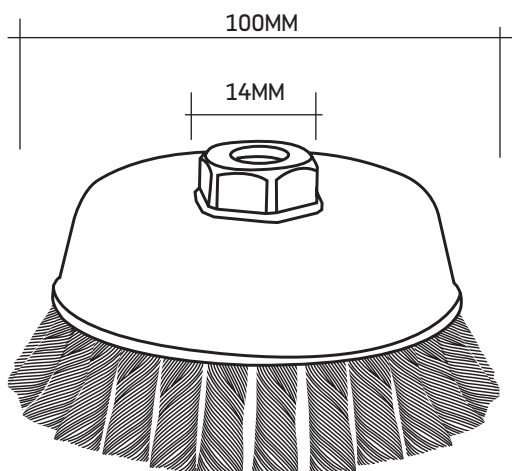
SAUCER KNOTTED WIRE
