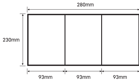
A. 1/3 sheet sander, cut as shown
